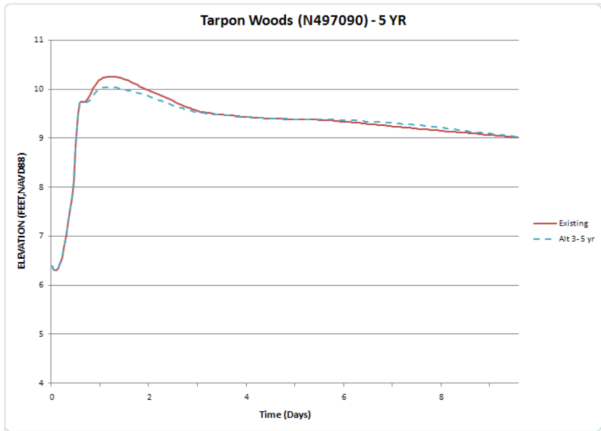
Figure 3.3.3c: Flood duration in Tarpon Woods, Alternative 3
