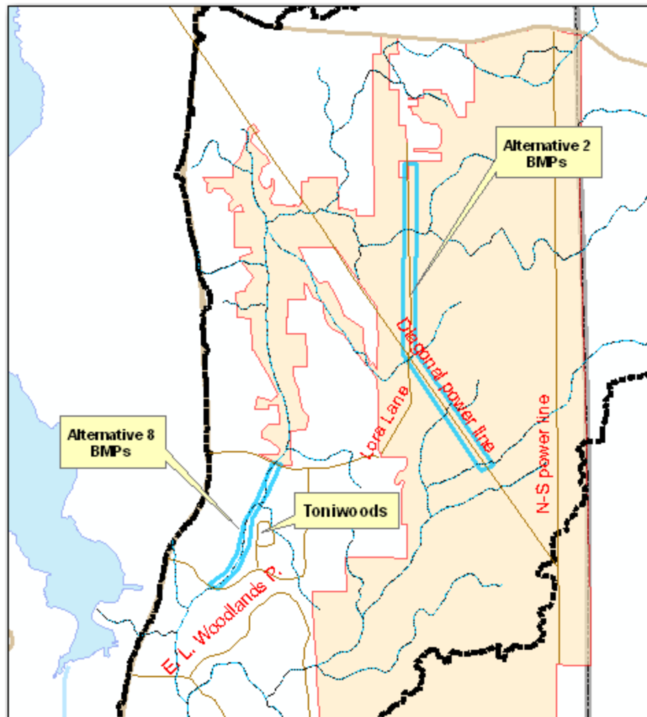
Figure 1.0c: BMP Alternative C2
