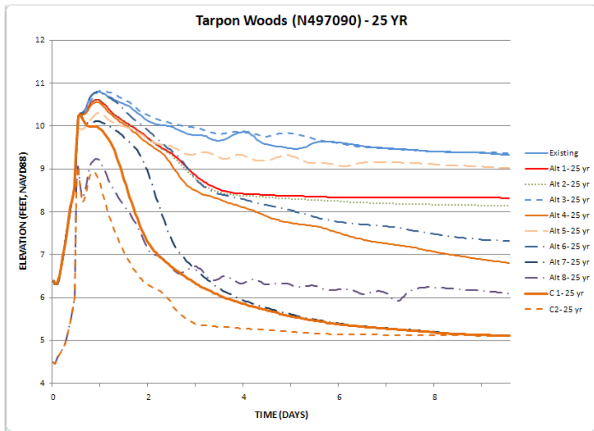
Figure 4.3: Comparison of duration of flooding in the Tarpon Woods area – 25 year, 24 hour event.
