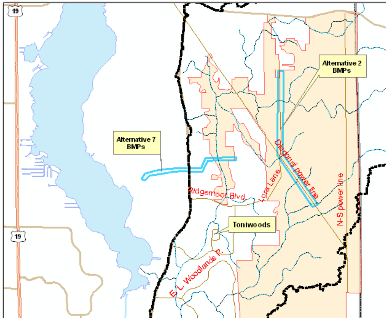
Figure 3.3.12a: Alternative C1 BMPs
