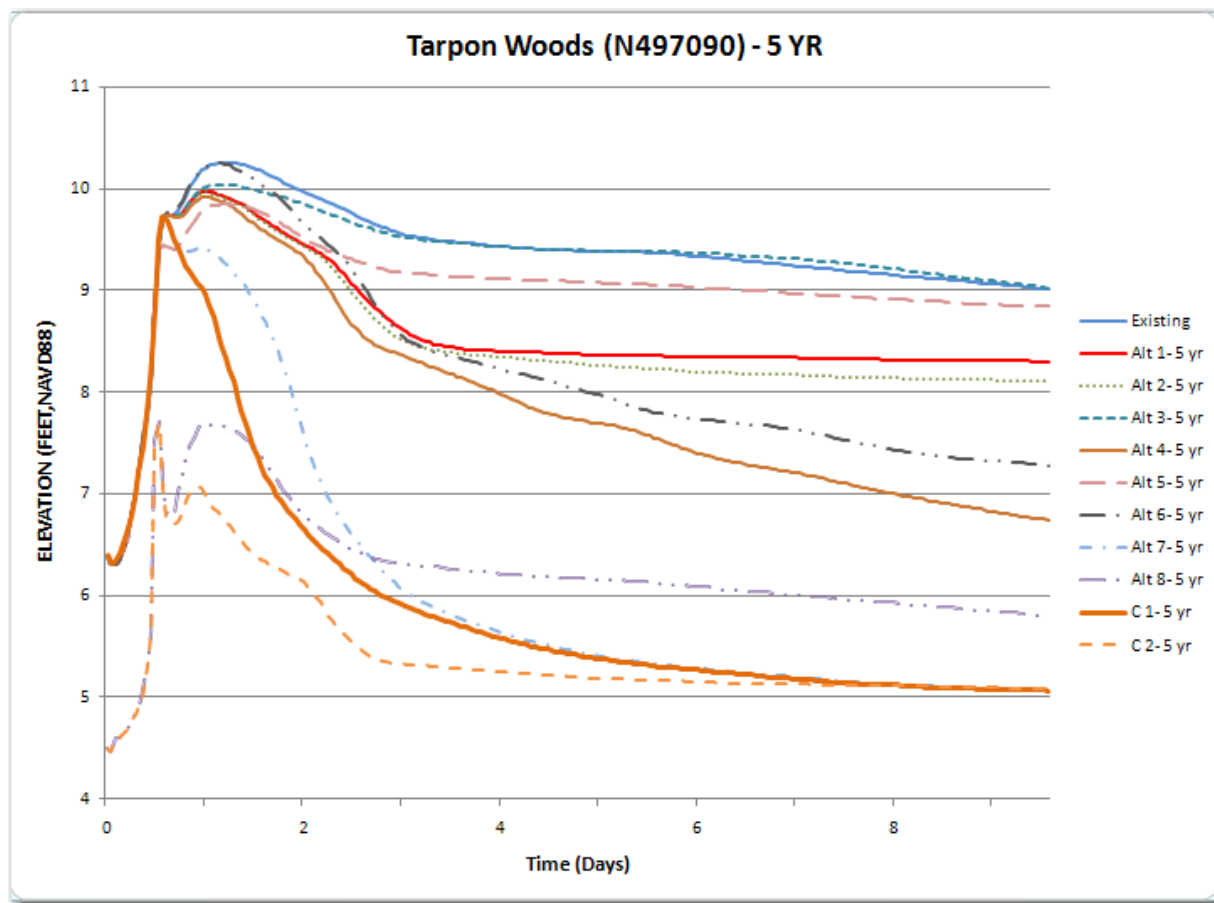
Figure 4.2: Duration of flooding in the Tarpon Woods area - 5 year, 24 hour event.
