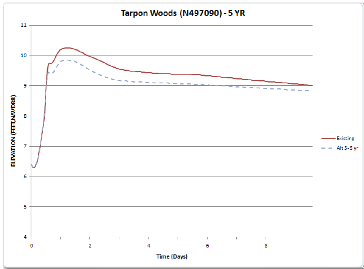
Figure 3.3.5b: Flood duration in Tarpon Woods, Alternative 5
