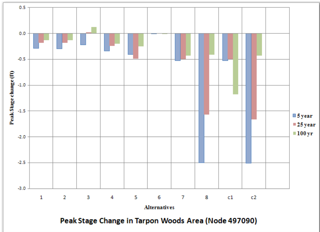
Figure 4.4: Comparison of alternative stage reductions in the Tarpon Woods area
