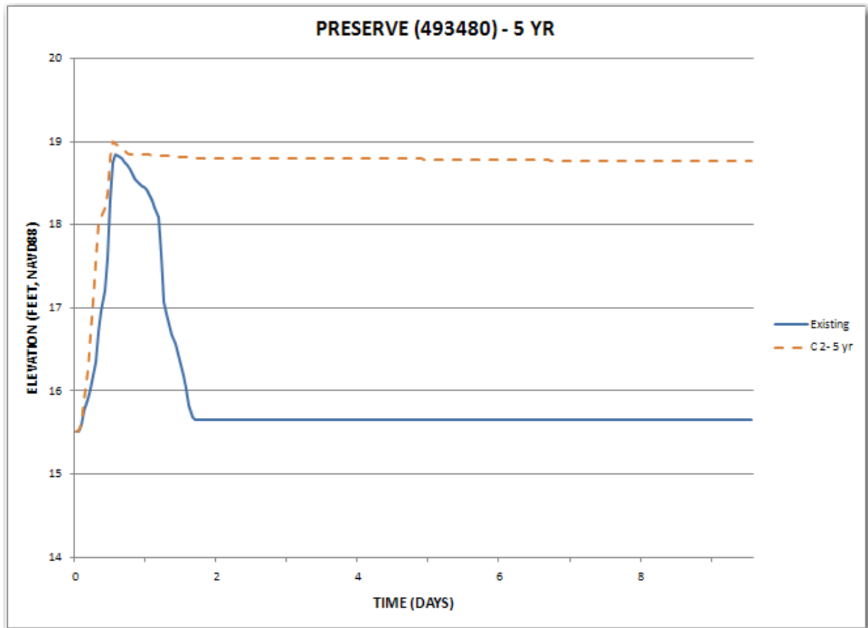
Figure 3.3.13c: Flood duration in Preserve, Alternative C2
