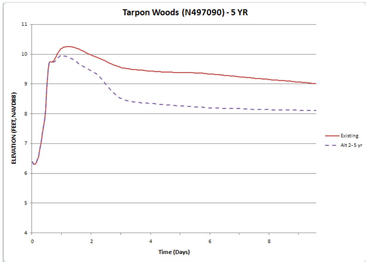
Figure 3.3.2c: Flood duration in Tarpon Woods, Alternative 2
