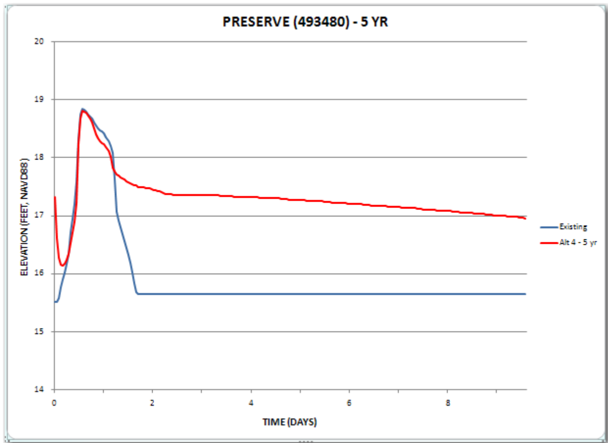
Figure 3.3.4b: Flood duration in Preserve, Alternative 4
