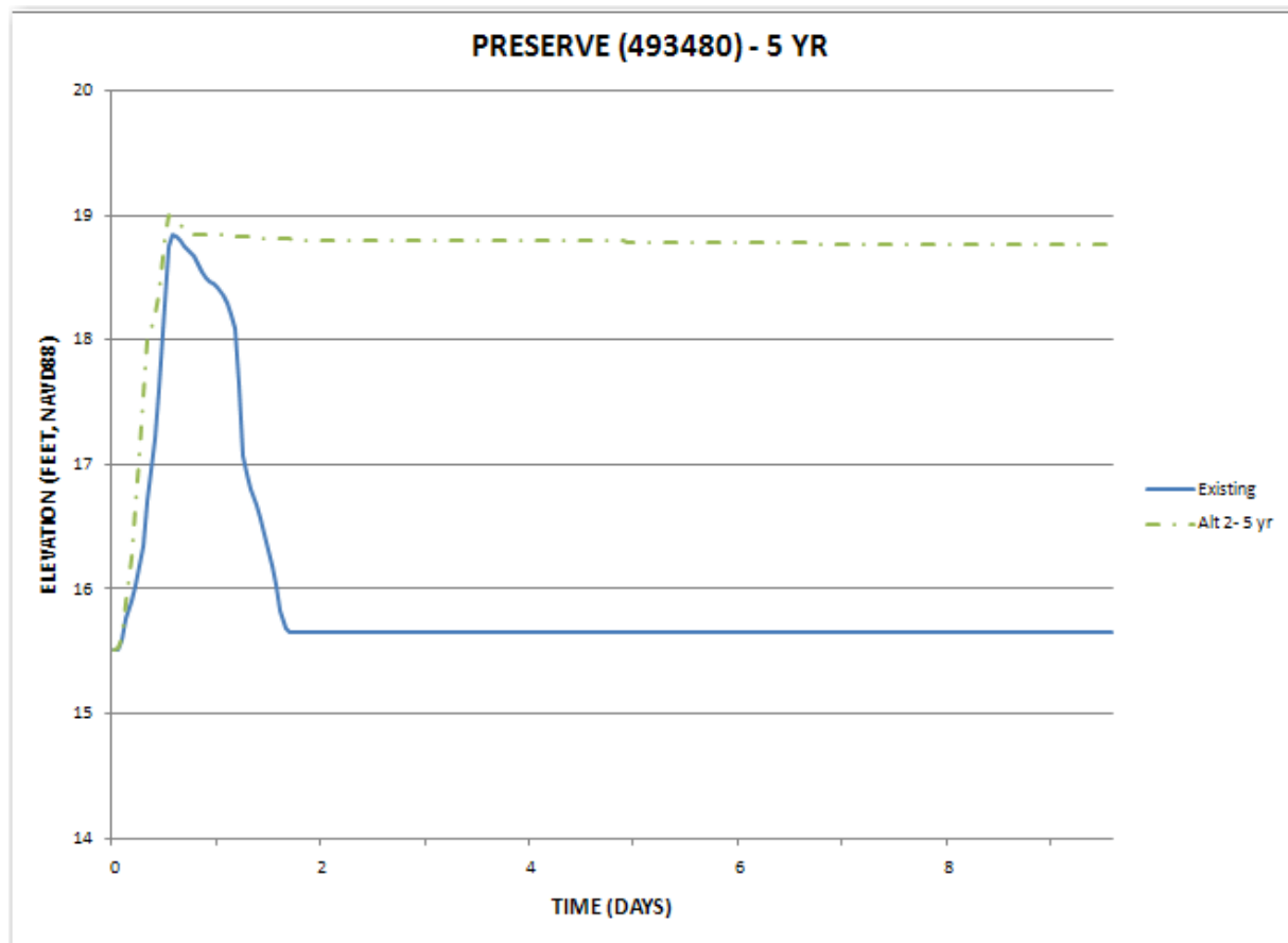
Figure 3.3.2b: Flood duration in Preserve, Alternative 2
