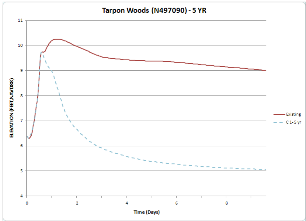
Figure 3.3.13b: Flood duration in Tarpon Woods, Alternative C2
