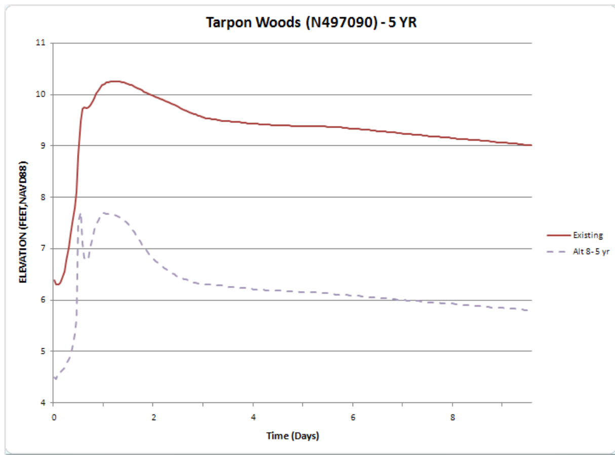
Figure 3.3.8b: Flood duration in Tarpon Woods, Alternative 8
