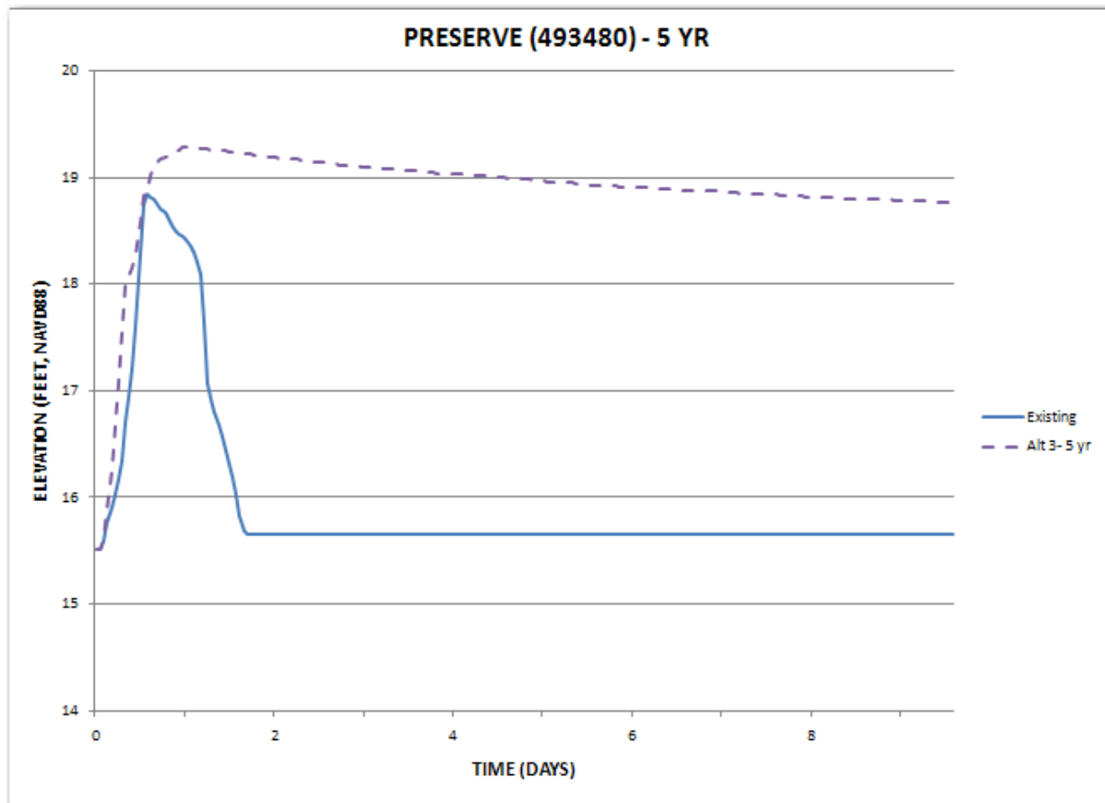
Figure 3.3.3b: Flood duration in Preserve, Alternative 3
