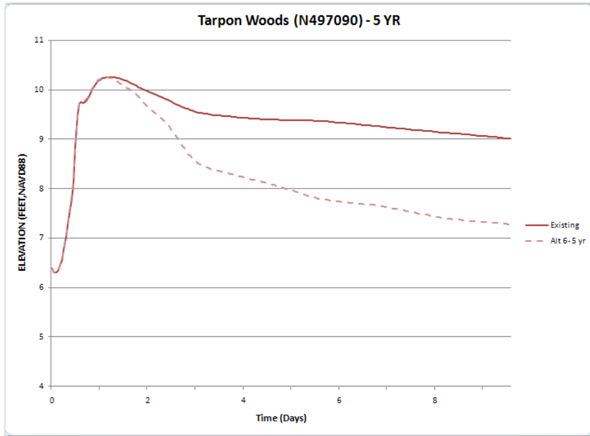
Figure 3.3.6b: Flood duration in Tarpon Woods, Alternative 6
