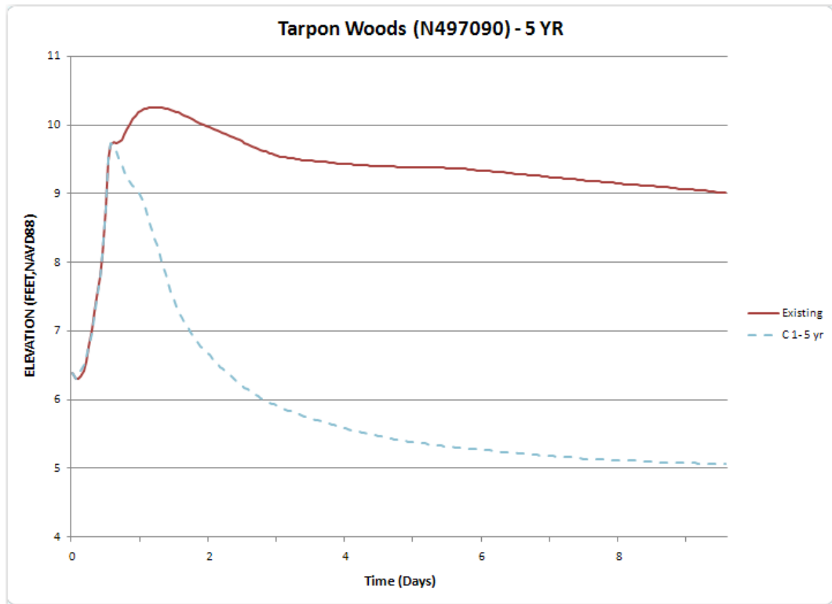
Figure 3.3.12c: Flood duration in Tarpon Woods, Alternative C1
