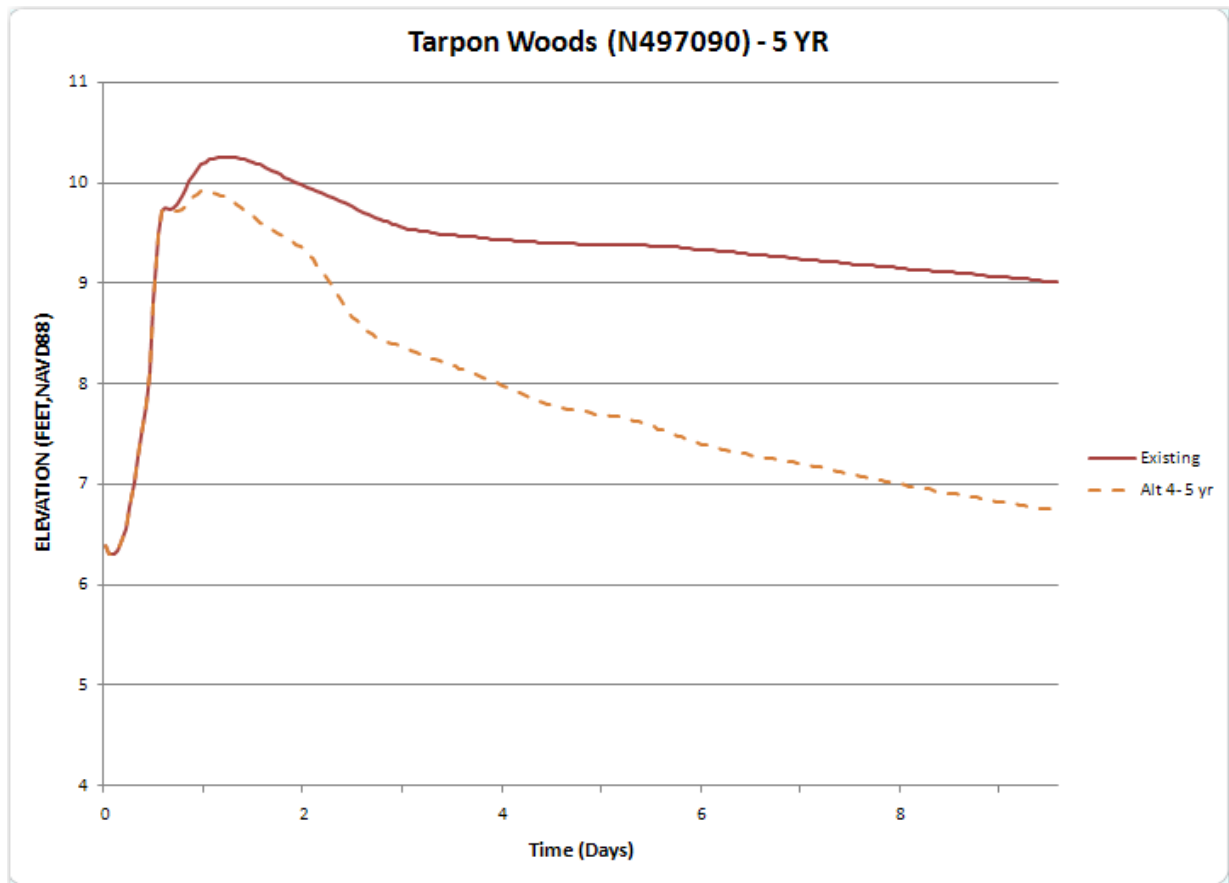
Figure 3.3.4c: Flood duration in Tarpon Woods, Alternative 4
