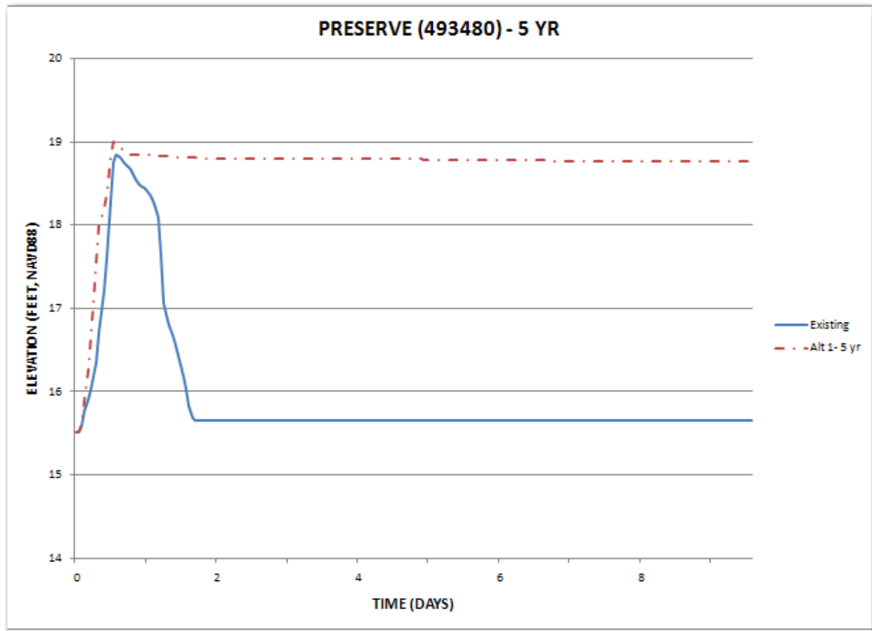
Figure 3.3.1b: Flood duration in Preserve, Alternative 1
