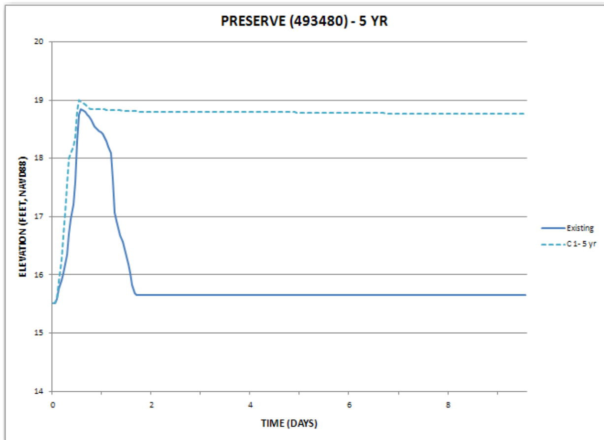
Figure 3.3.12b: Flood duration in Preserve, Alternative C1
