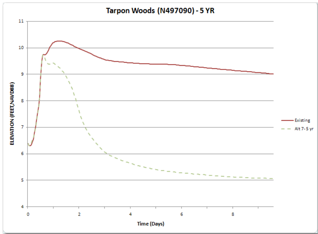
Figure 3.3.7b: Flood duration in Tarpon Woods, Alternative 7
