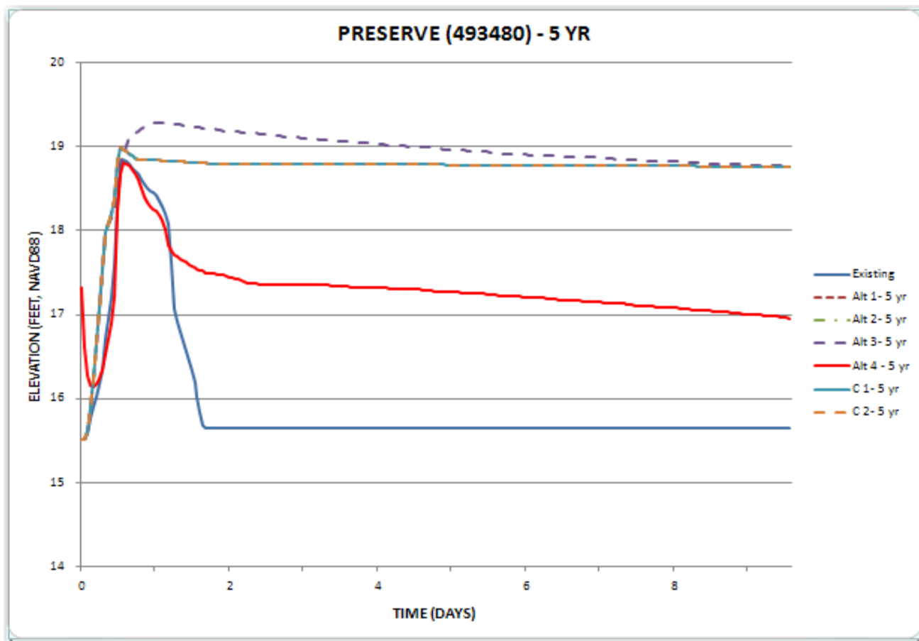
Figure 4.1: Duration of flooding in the Preserve area - 5 year, 24 hour event.
