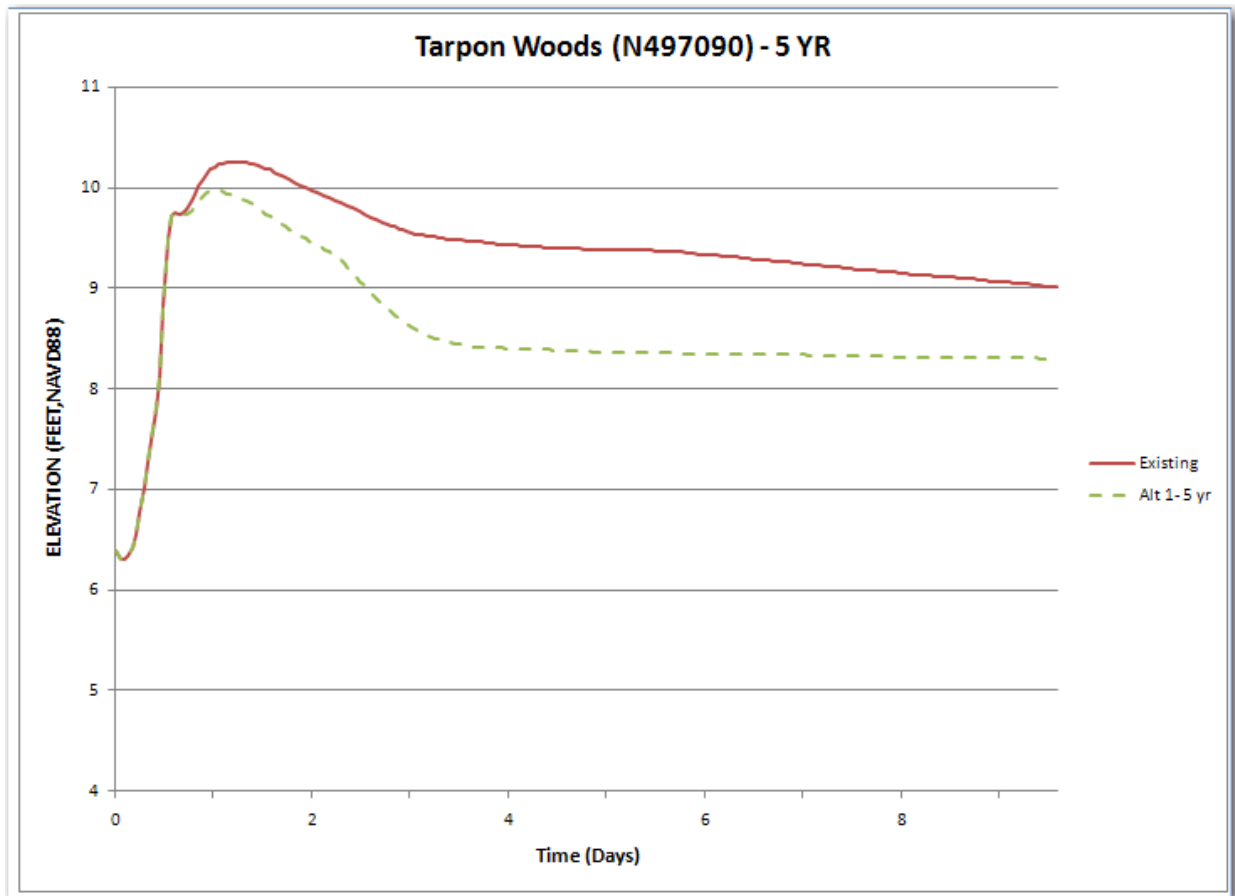
Figure 3.3.1c: Flood duration Tarpon Woods Area, Alternative 1
